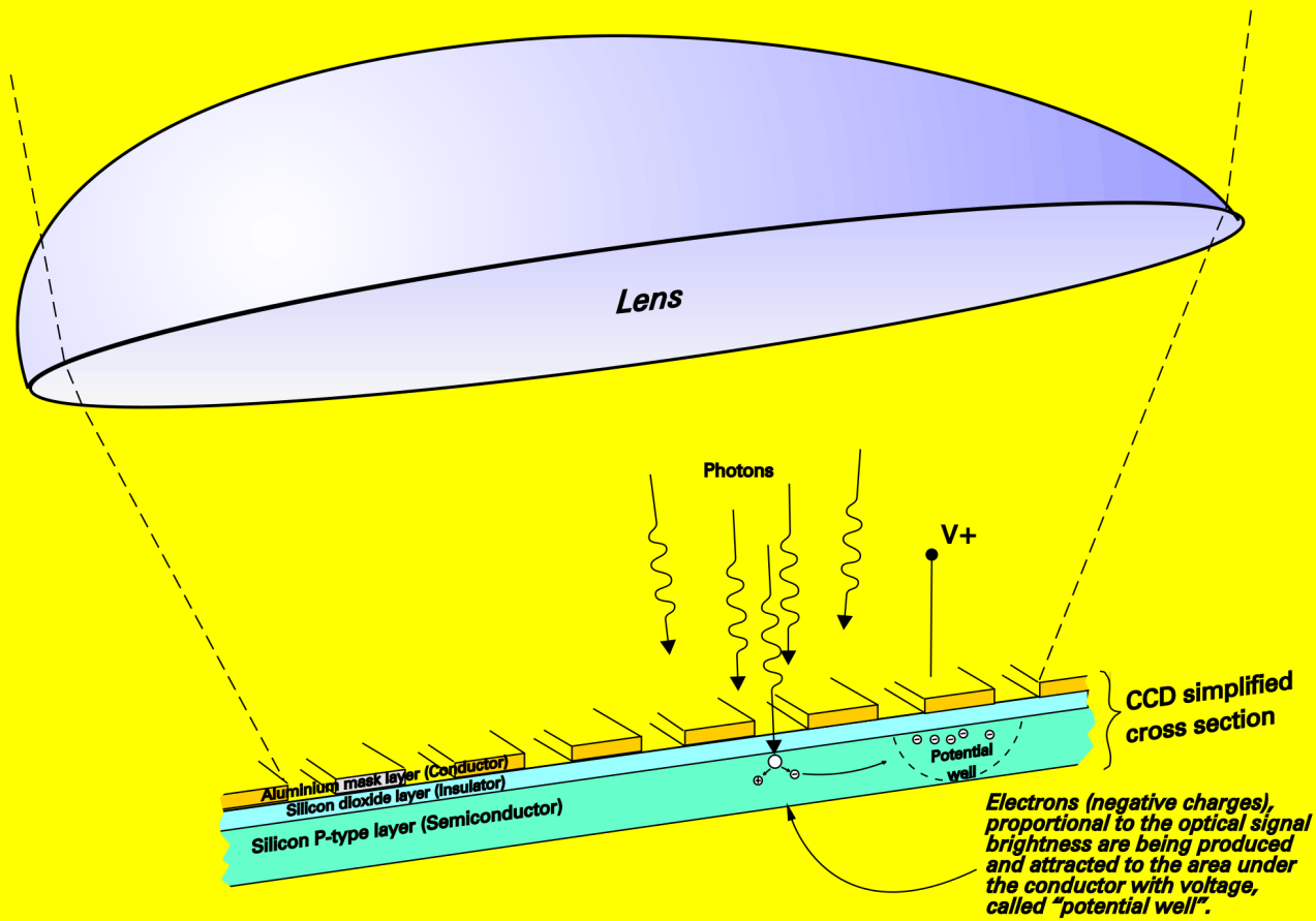
Electrons in a CCD chip are generated by photons
